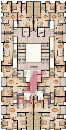
BLOCK - B FIRST FLOOR PLAN
